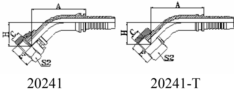
45°公制内螺纹平面 45° METRIC FEMALE FLAT SEAT
